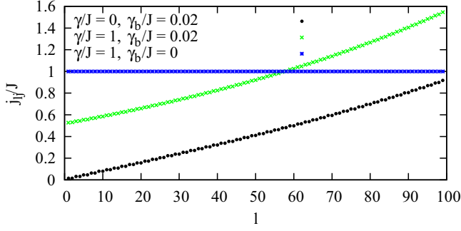
FIG. 6. The currents j_{i,i+1} between nearest-neighbor sites along the x direction for the source-drain setup (7). Parameters used: F/J = 1 , \Delta/J = -2 .
