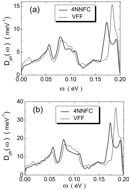
FIG. 2. The phonon density of states for the (a) \{L=9, R=5\} and (b) \{L=13, R=7\} graphene antidot lattices, obtained using the 4NNFC (solid line) and VFF (dashed line) methods.
