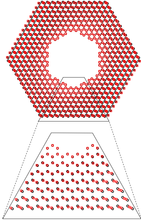
FIG. 3. (Color online) The atomic displacement pattern corresponding to the zone-center phonon mode at energy E_\lambda \approx 197.5 meV of the \{L=13, R=5\} graphene antidot lattice (top) and its zoomed version (bottom). The displaced (undisplaced) atomic positions are designated by the squares (dark circles).
