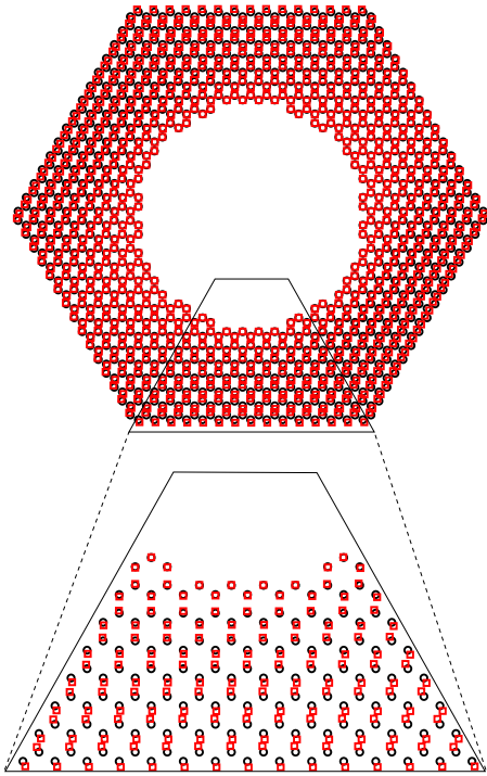
FIG. 4. (Color online) The atomic displacement pattern corresponding to the zone-center phonon mode at energy E_\lambda \approx 197.5 meV of the \{L=15, R=7\} graphene antidot lattice (top) and its zoomed version (bottom). The displaced (undisplaced) atomic positions are designated by the squares (dark circles).
