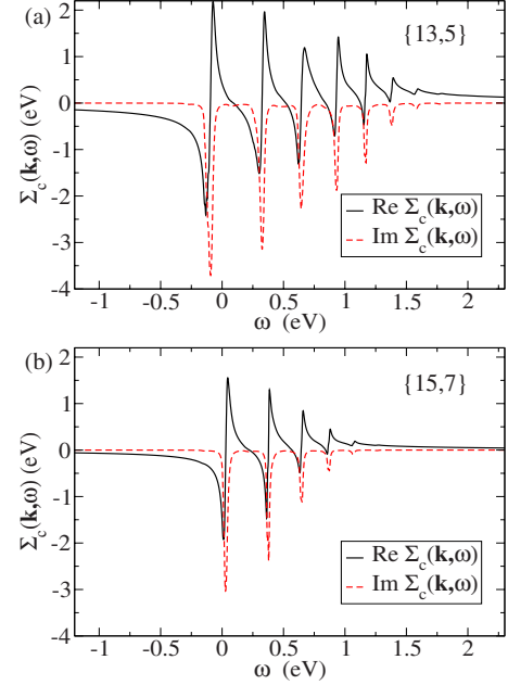
FIG. 7. (Color online) The real and imaginary parts of the SCBA conduction-band electron self-energy in the (a) \{L=13, R=5\} and (b) \{L=15, R=7\} graphene antidot lattices for \mathbf{k}=0.2 \mathbf{b} , where \mathbf{b}=(0, 1)*4\pi/(3La) .
