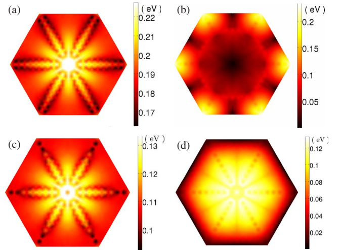
FIG. 5. (Color online) The \mathbf{q} dependence of the moduli |\gamma_{cc}^\lambda(\mathbf{k}=0, \mathbf{q})| of the bare e-ph vertex functions, for selected high-energy phonon branches \lambda , in the hexagonal Brillouin zones of the \{L=13, R=5\} [(a) and (b)] and \{L=15, R=7\} [(c) and (d)] graphene antidot lattices. The energies of the corresponding optical phonons at \mathbf{q}=0 , as obtained using the VFF approach, are E_\lambda \approx 197.5 meV [(a), (c), and (d)] and E_\lambda \approx 197.4 meV [(b)].
