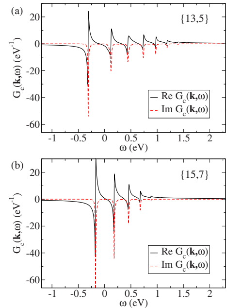
FIG. 8. (Color online) The SCBA electron propagators in the (a) \{L=13, R=5\} and (b) \{L=15, R=7\} graphene antidot lattices for \mathbf{k}=0.2 \mathbf{b} , where \mathbf{b}=(0, 1)*4\pi/(3La) .
