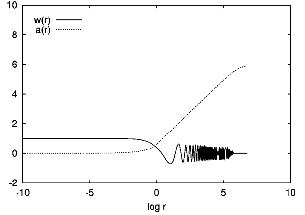
FIG. 2. Solution for the parameters w_2 = -10 , a_1 = 0.5 and integration step h = 10^{-3} . The initial point of integration is r_i = 10^{-10} .
