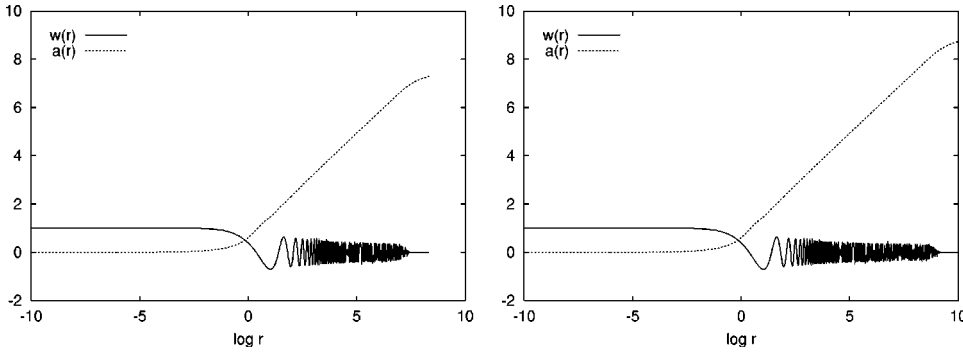
FIG. 3. Solutions for parameters w_2 = -10 , a_1 = 0.5 , r_i = 10^{-10} and integration steps h = 10^{-4} (left) and h = 10^{-5} (right).
