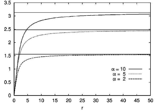
FIG. 1. Dyon solution for various values of \alpha .
